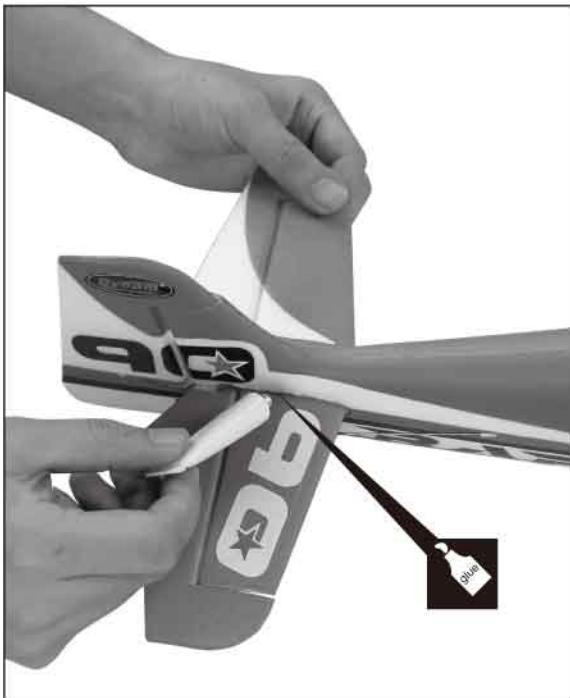
3 Apply some glue on the area of contact for the stabilizer. Glue the stabilizer in place.
